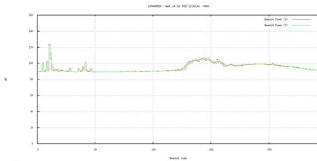
Beamlets
