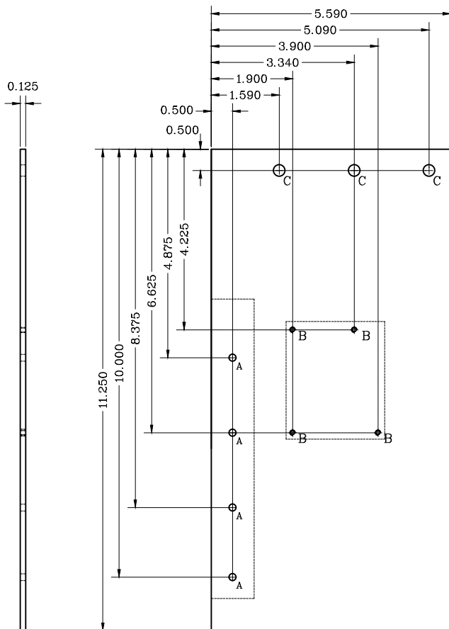
TLC MAIN PANEL, 5 REQUIRED
