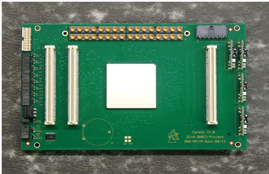
Fig. 3: Prototype of the CORE3-L board. In the centre the FPGA can be seen. The connectors for the high speed buses are visible on the left and right side. On the top are two rows of additional input connectors.
