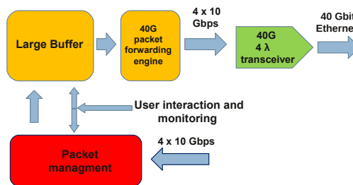
Figure 3: Block diagrams of the FILA40G unit. The data comes into the “packet management” subunit as 4 × 10 Gbps data streams. This subunit will handle additional data processing. Via the “large buffer” the data flows via the “40G packet forwarding engine” to a 40GE transceiver and on to Ethernet.
