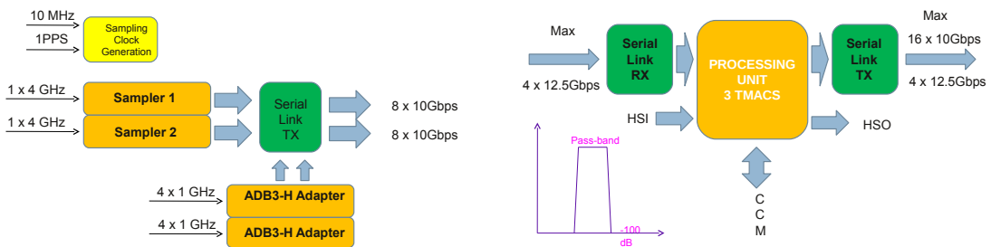
Figure 2: Block diagrams of the analogue-digital converter ADB3-L (left) and the processing unit CORE3-L (right). “HSI” is the high speed input bus, “HSO” high speed output bus, and “CCM” command, control and monitoring bus.
