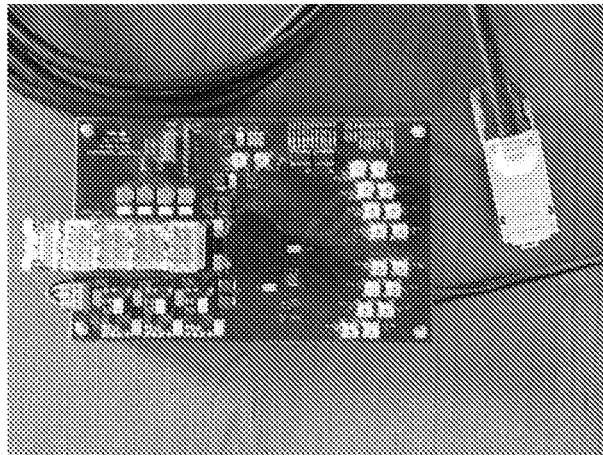
Figure 2. GLAPPER (glass to copper) prototype board to connect a DBBC with a MK5C
