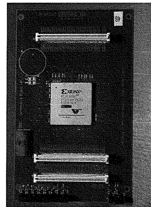
Fig. 3 The processing board CoreBoard1.
