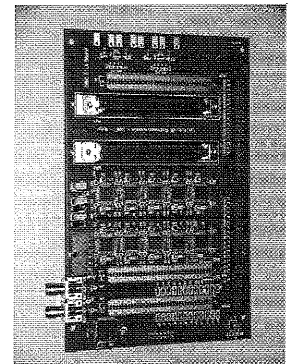
Fig. 4 The FiLa Board.
